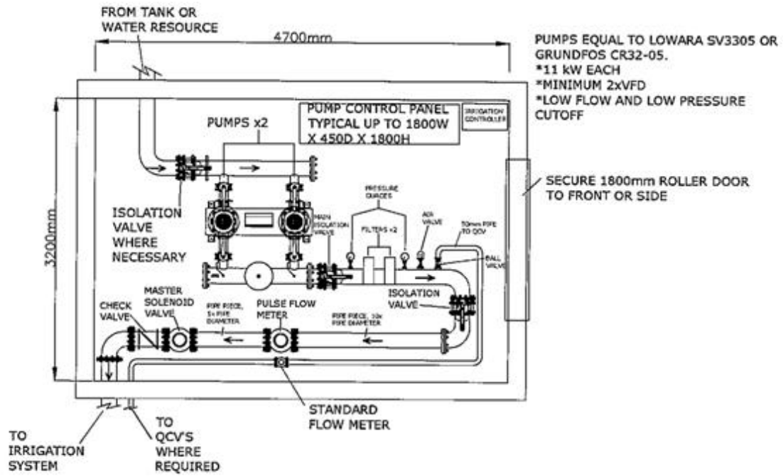
TYPICAL SCHEMATIC PUMP STATION PLAN TO NOMINAL 9Lt/Sec © COPYRIGHT 2018 TOTAL IRRIGATION DESIGNERS. –NO SCALE
