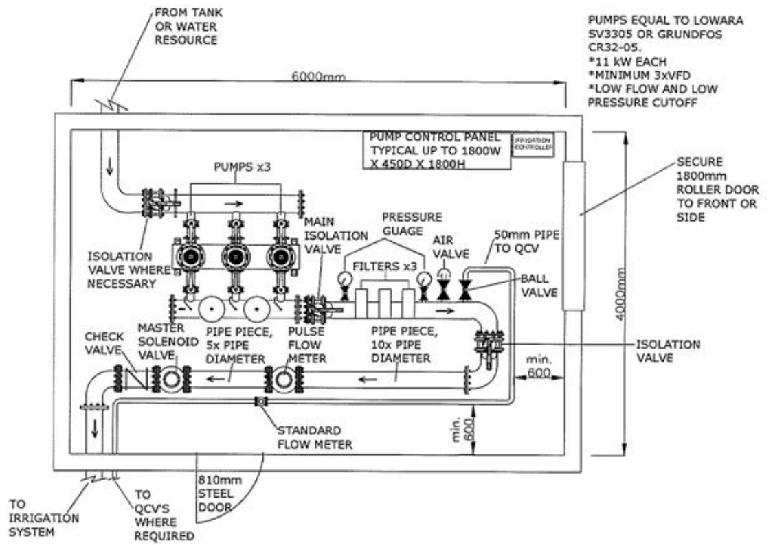
TYPICAL SCHEMATIC PUMP STATION PLAN TO NOMINAL 18Lt/Sec
