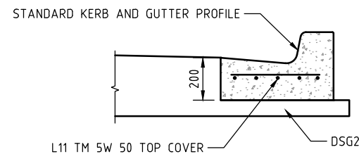
REINFORCED BUS STOP KERB AND GUTTER DETAIL N.T.S.
