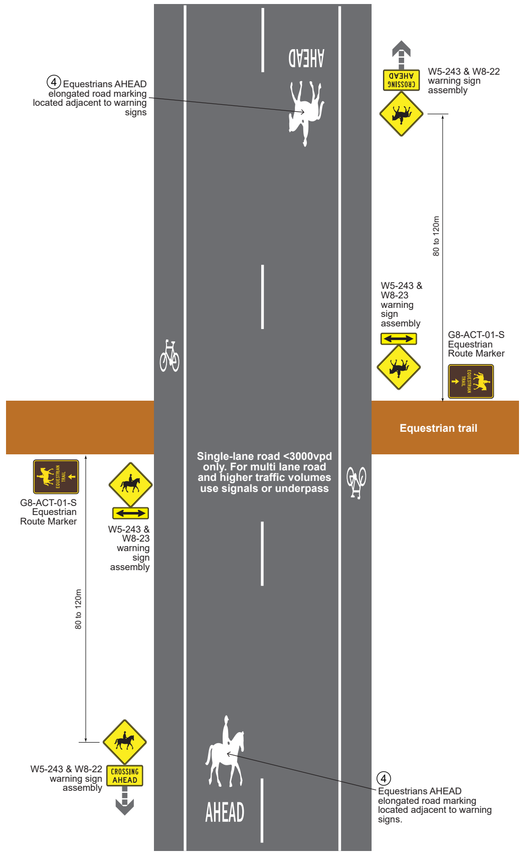
At-grade uncontrolled equestrian road crossing
