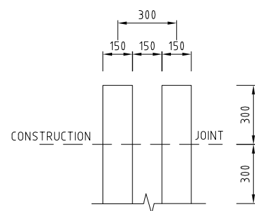
SPLICE BAR DETAIL B
