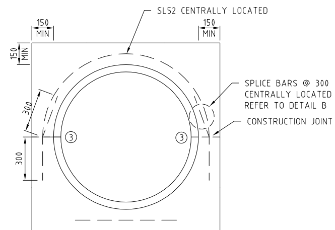
TYPICAL SECTION A
