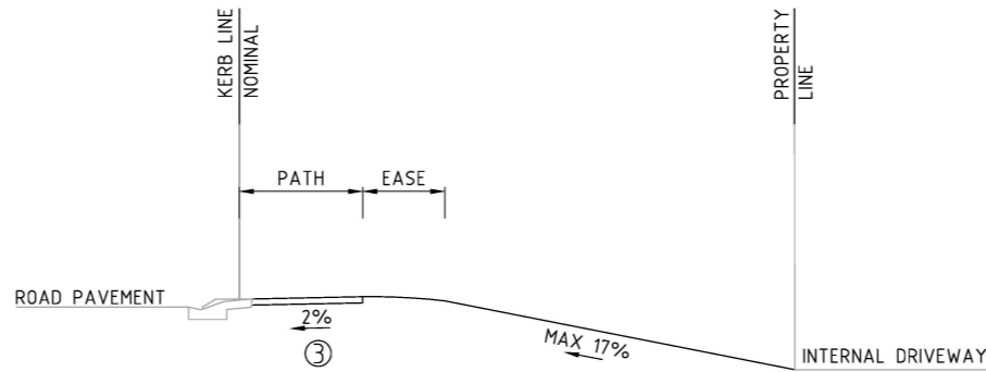
FALLING DRIVEWAY WITH PATH AT KERB
