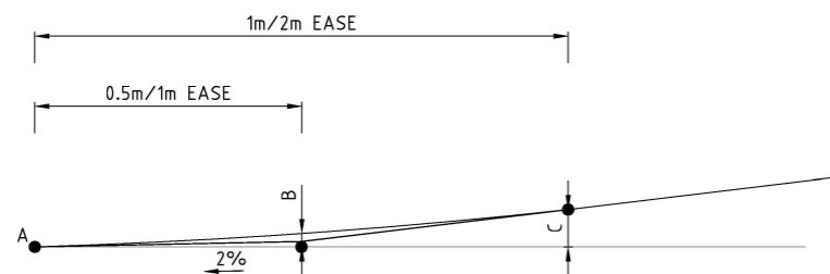
1m EASE RISING
