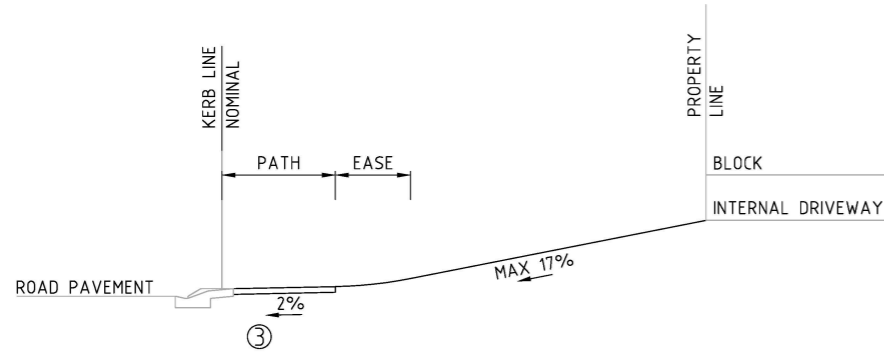
RISING DRIVEWAY WITH PATH AT KERB
