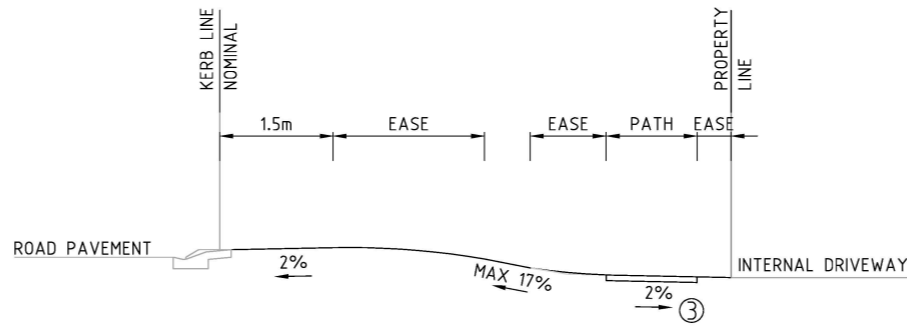
FALLING DRIVEWAY WITH PATH AT PROPERTY LINE
