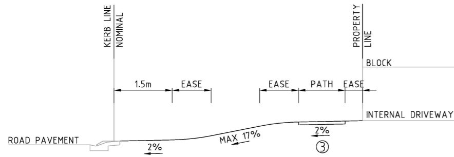
RISING DRIVEWAY WITH PATH AT PROPERTY LINE
