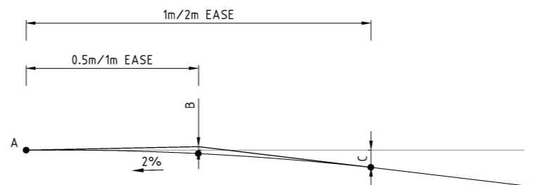
1m EASE FALLING
