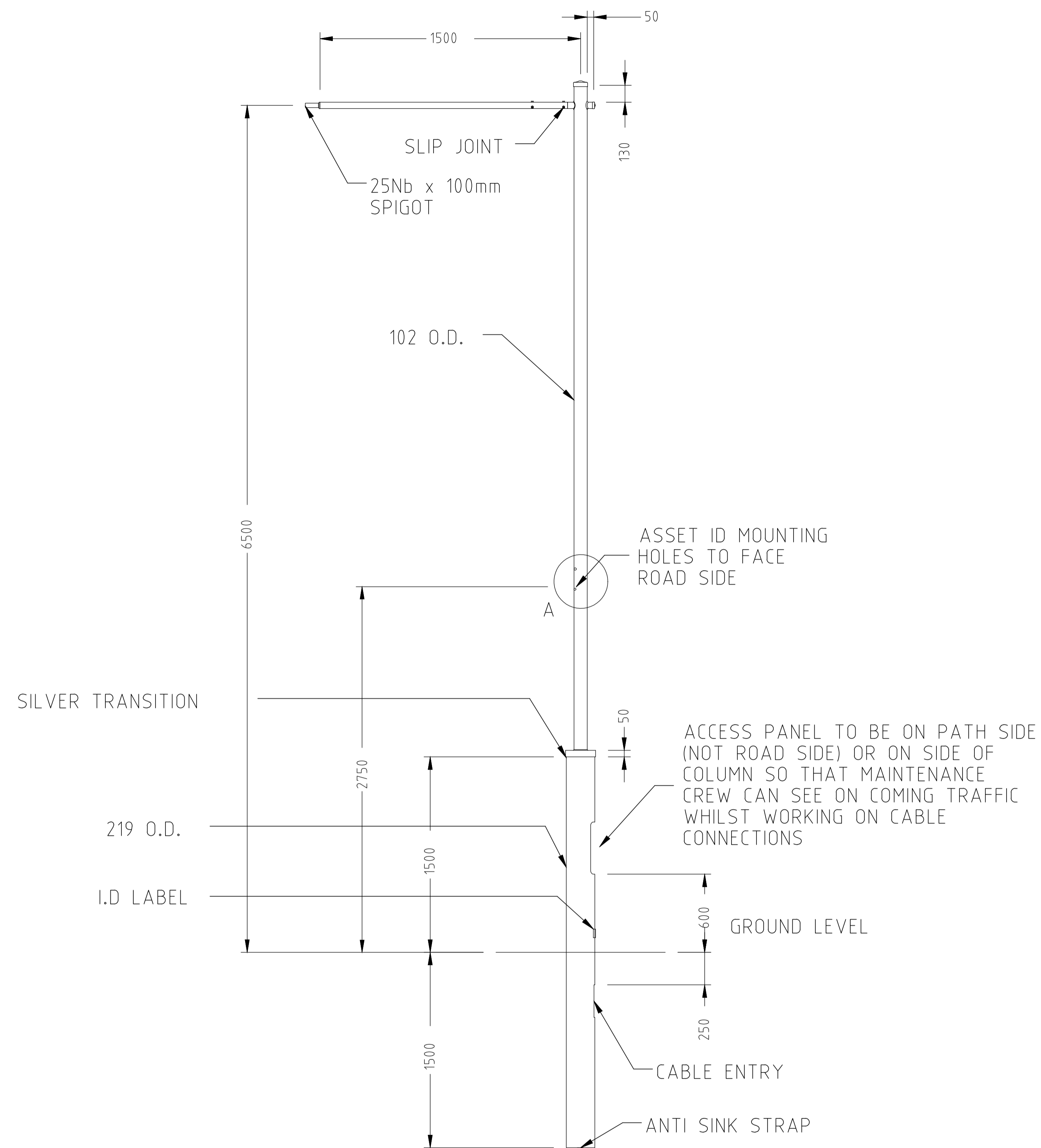
SIDE VIEW
