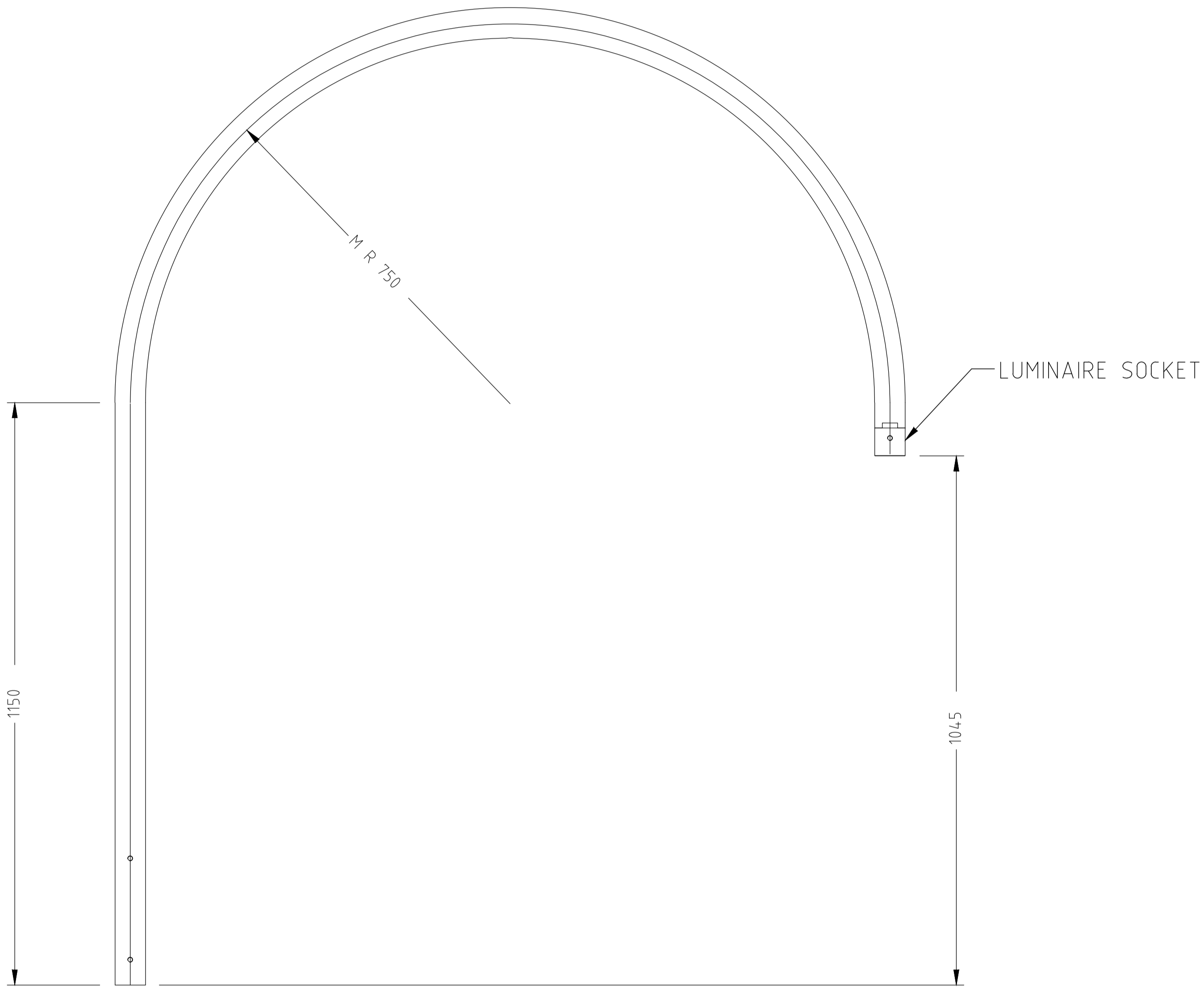
SIDE ELEVATION
