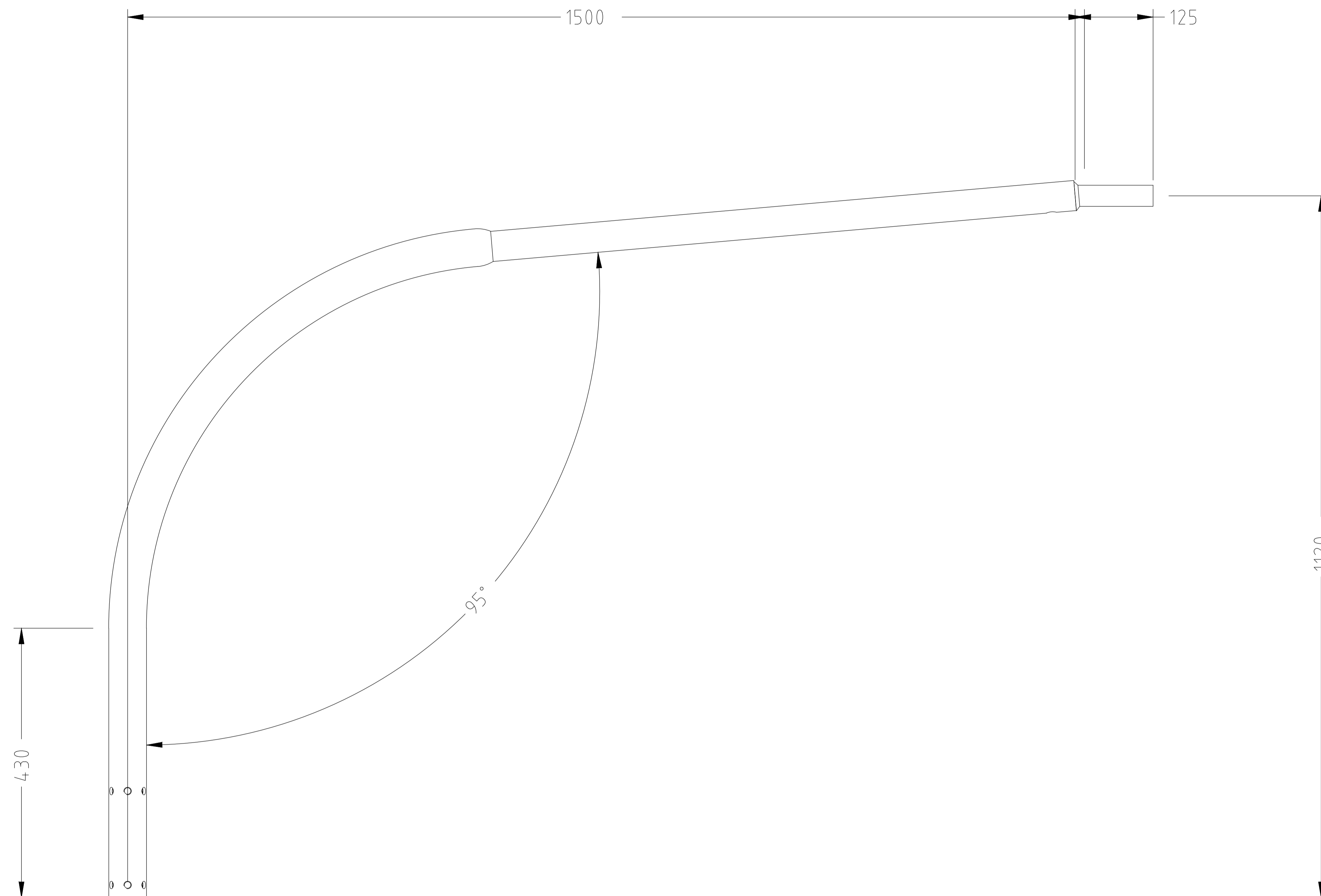
SIDE ELEVATION
