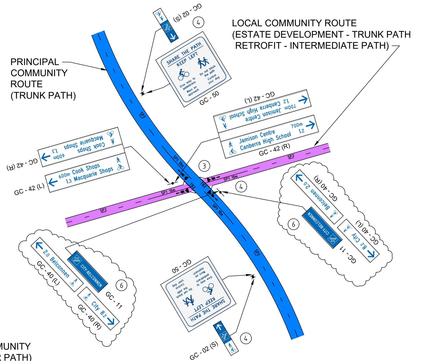
PRINCIPAL / MAIN COMMUNITY ROUTE (P/MCR) CROSS INTERSECTION WITH LOCAL COMMUNITY ROUTE (LCR)
