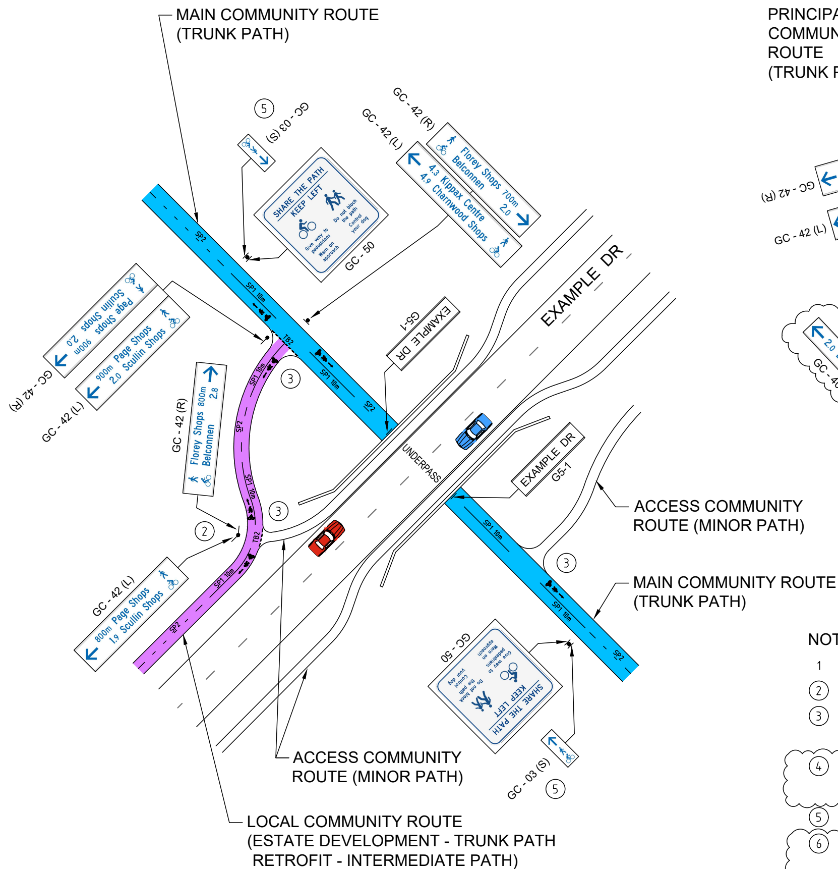
PRINCIPAL / MAIN COMMUNITY ROUTE (P/MCR) INTERSECTION WITH LOCAL COMMUNITY ROUTE (LCR) NEAR AN UNDERPASS
