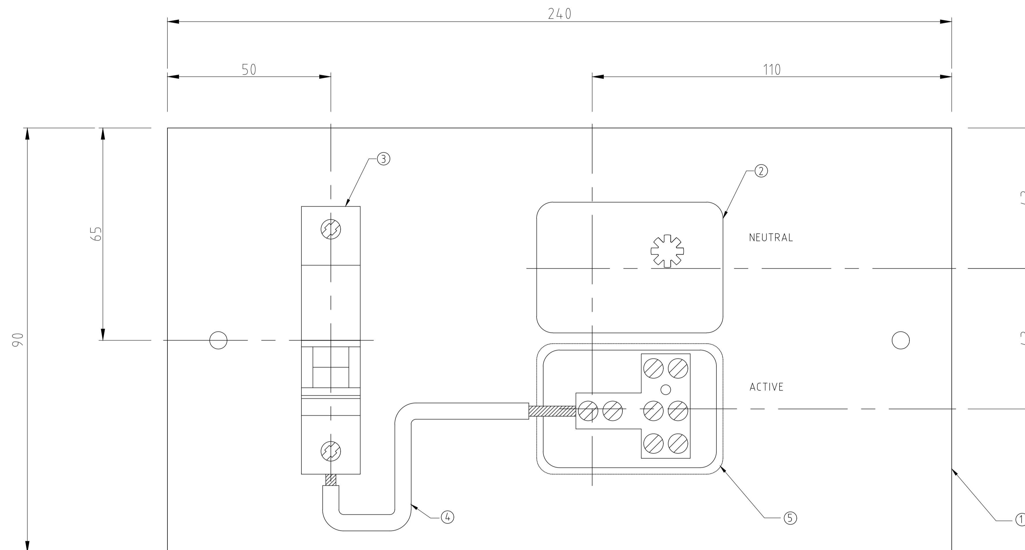
COMPLETE ASSEMBLY
