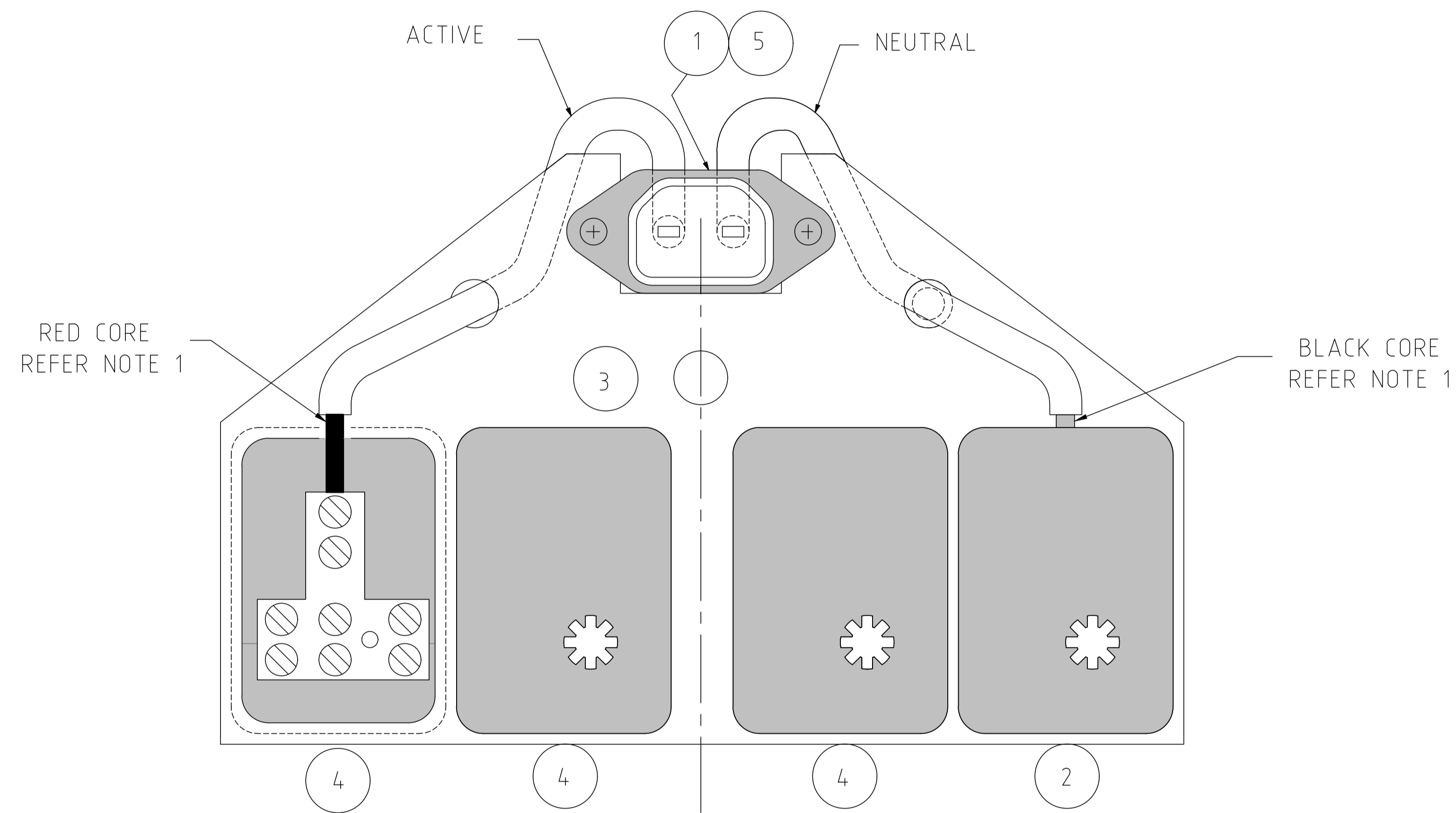
WIRING DIAGRAM
