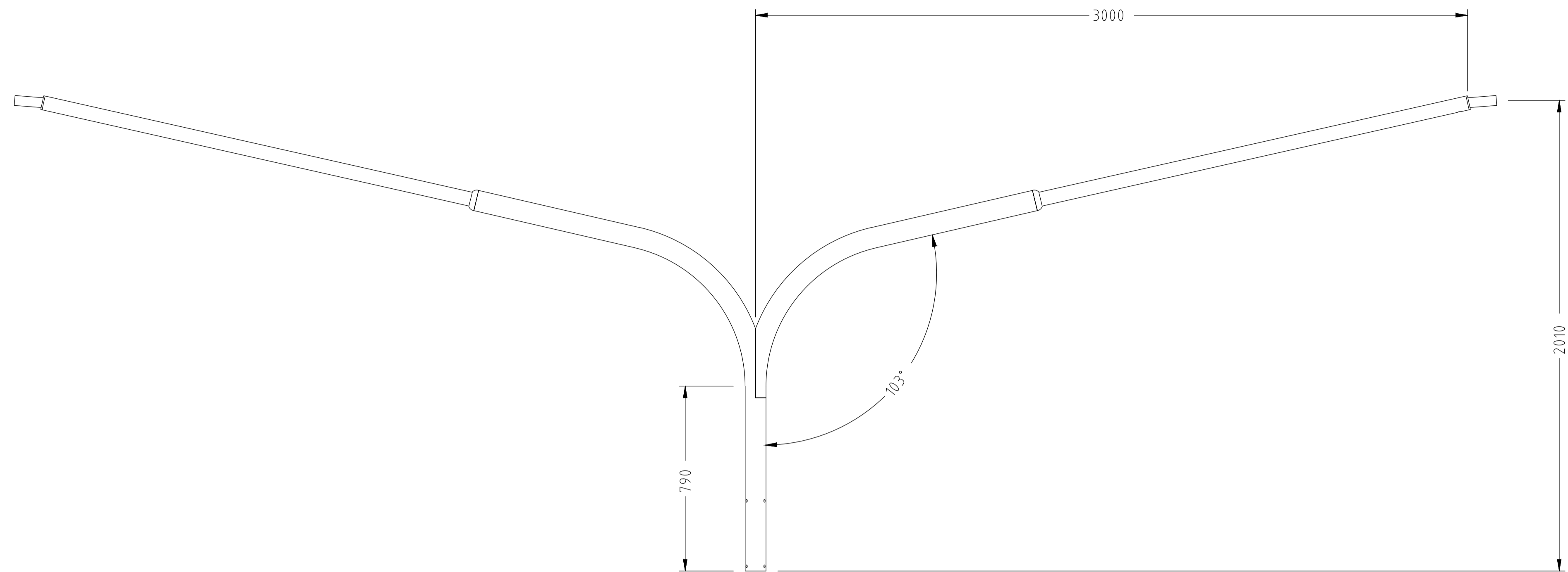
SIDE ELEVATION
