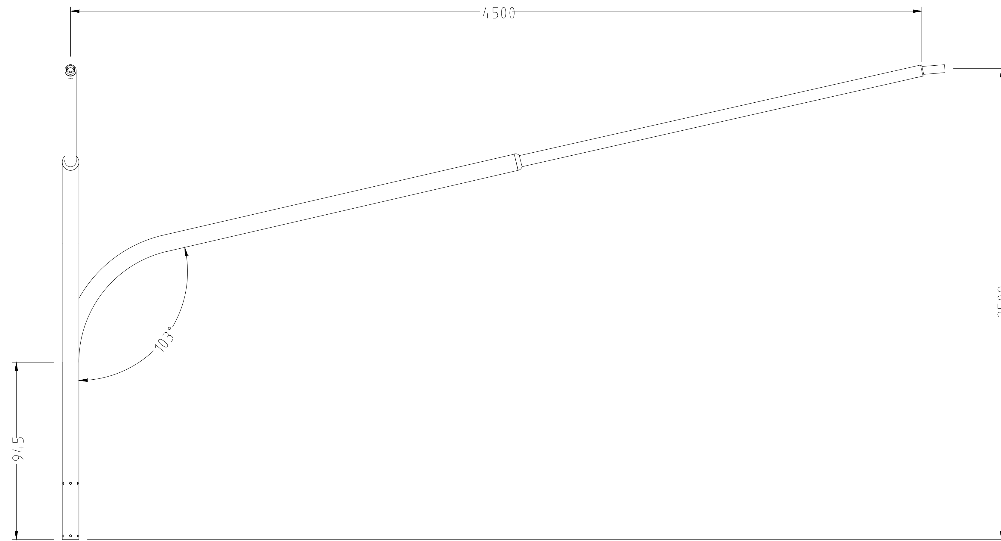
SIDE ELEVATION
