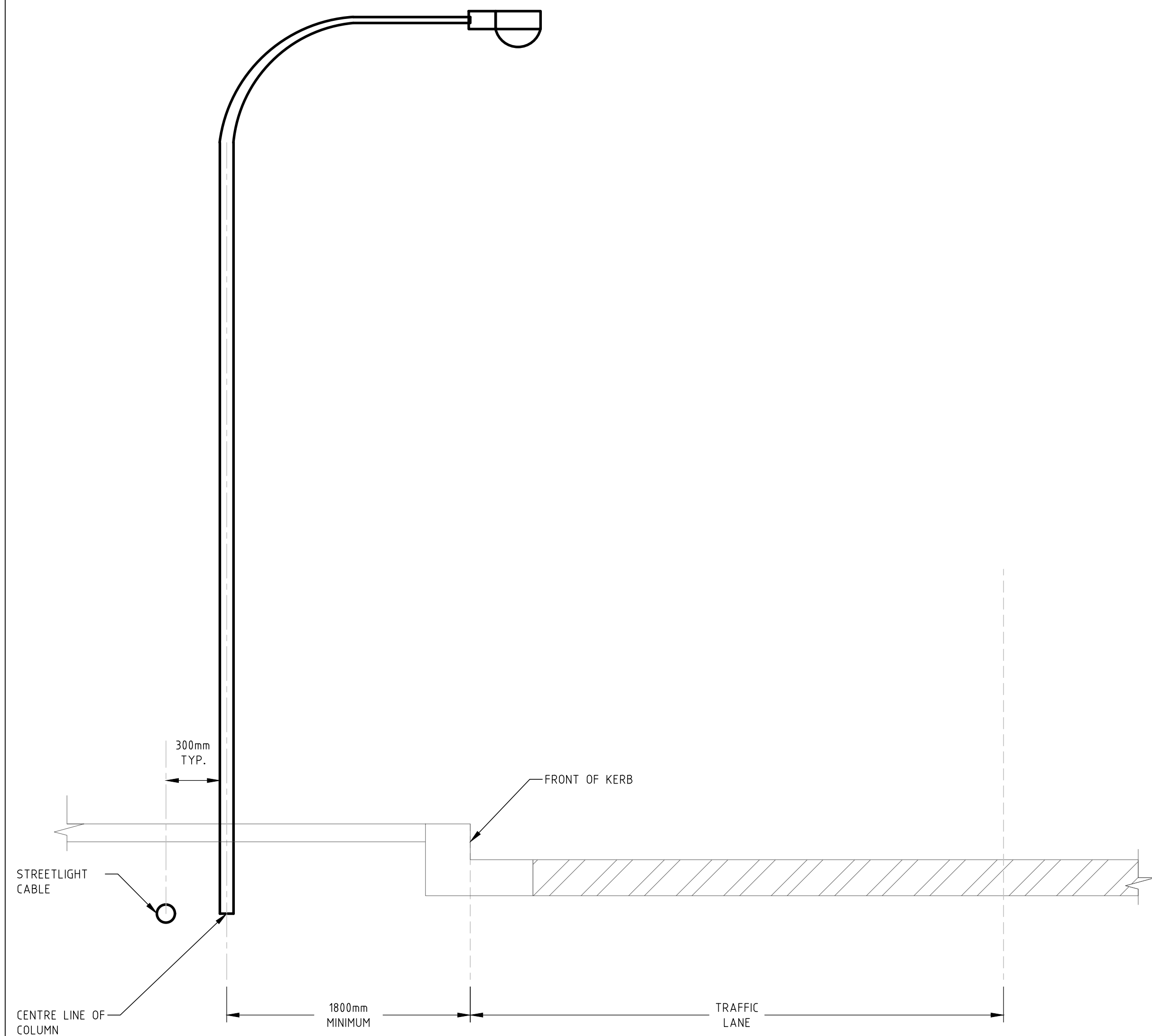
KERBED ROAD DIRECT BURIED IMPACT ABSORBING COLUMNS
