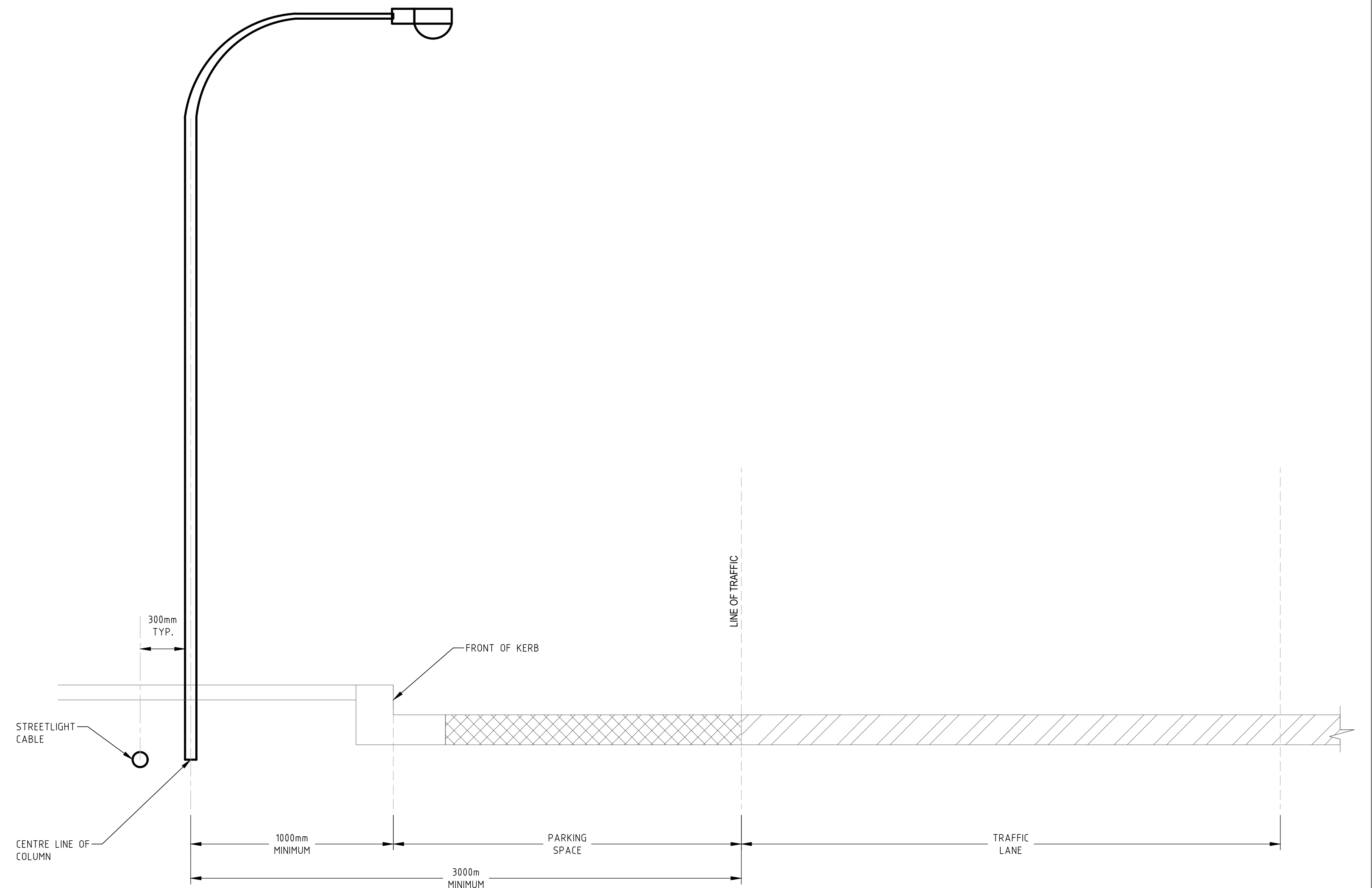
KERBED ROAD WITH STOPPING OR CYCLE LANE DIRECT BURIED IMPACT ABSORBING COLUMNS
