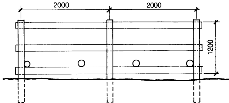
SIDE ELEVATION
