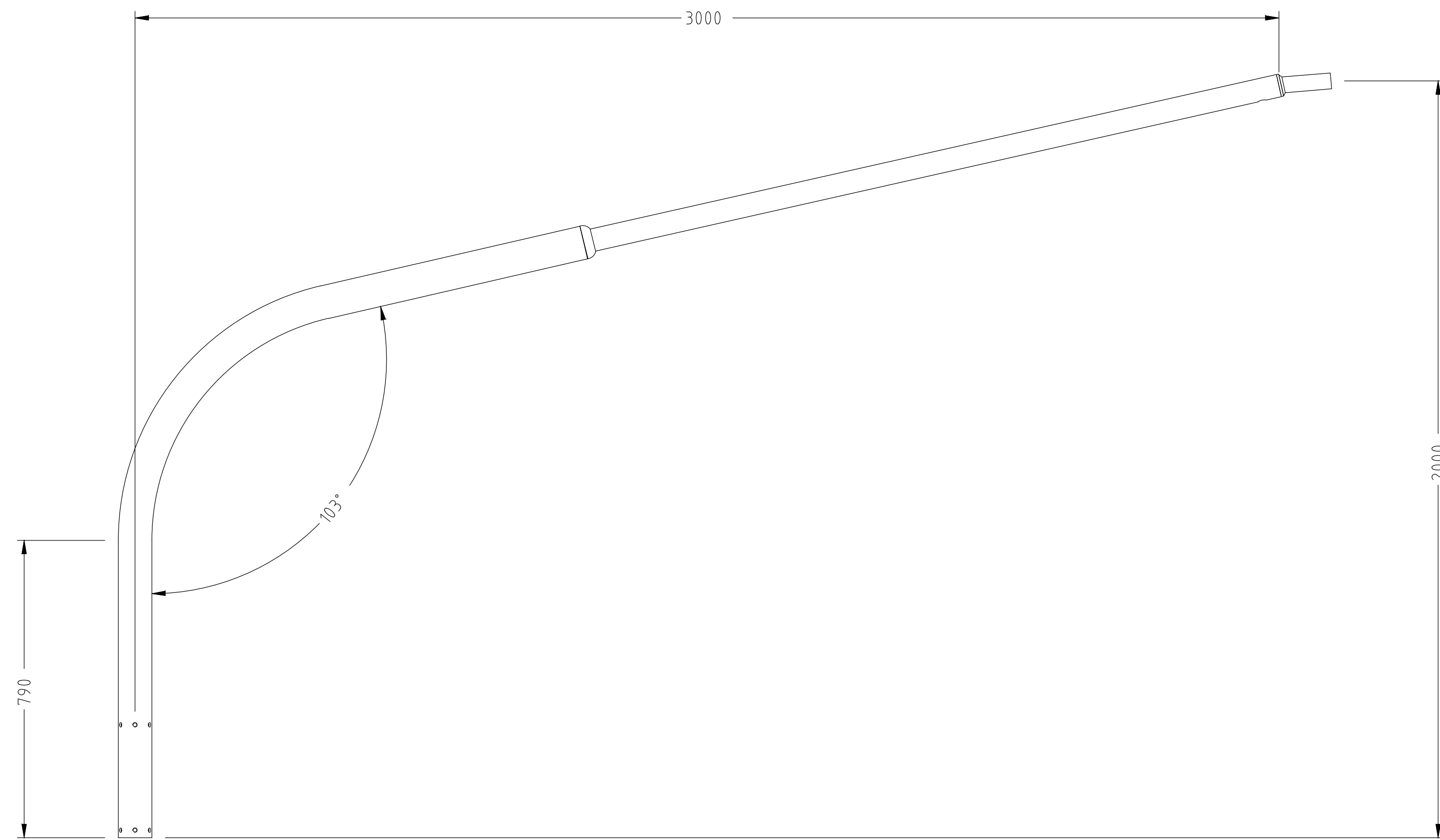
SIDE ELEVATION
