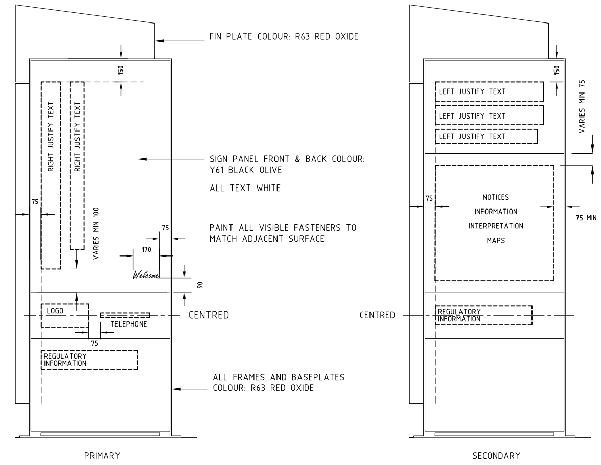
FINISHES & TYPICAL GRAPHIC LAYOUT 1:25
