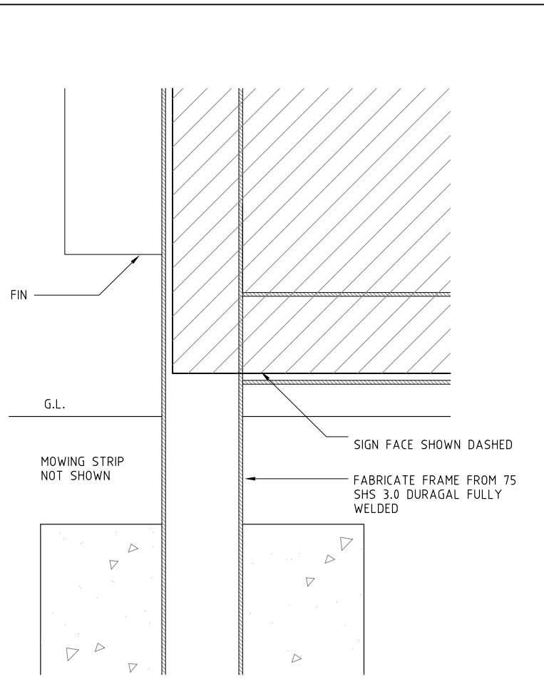
DETAIL SECTION 1:5
