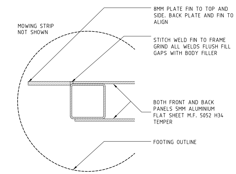
DETAIL PLAN 1:5
