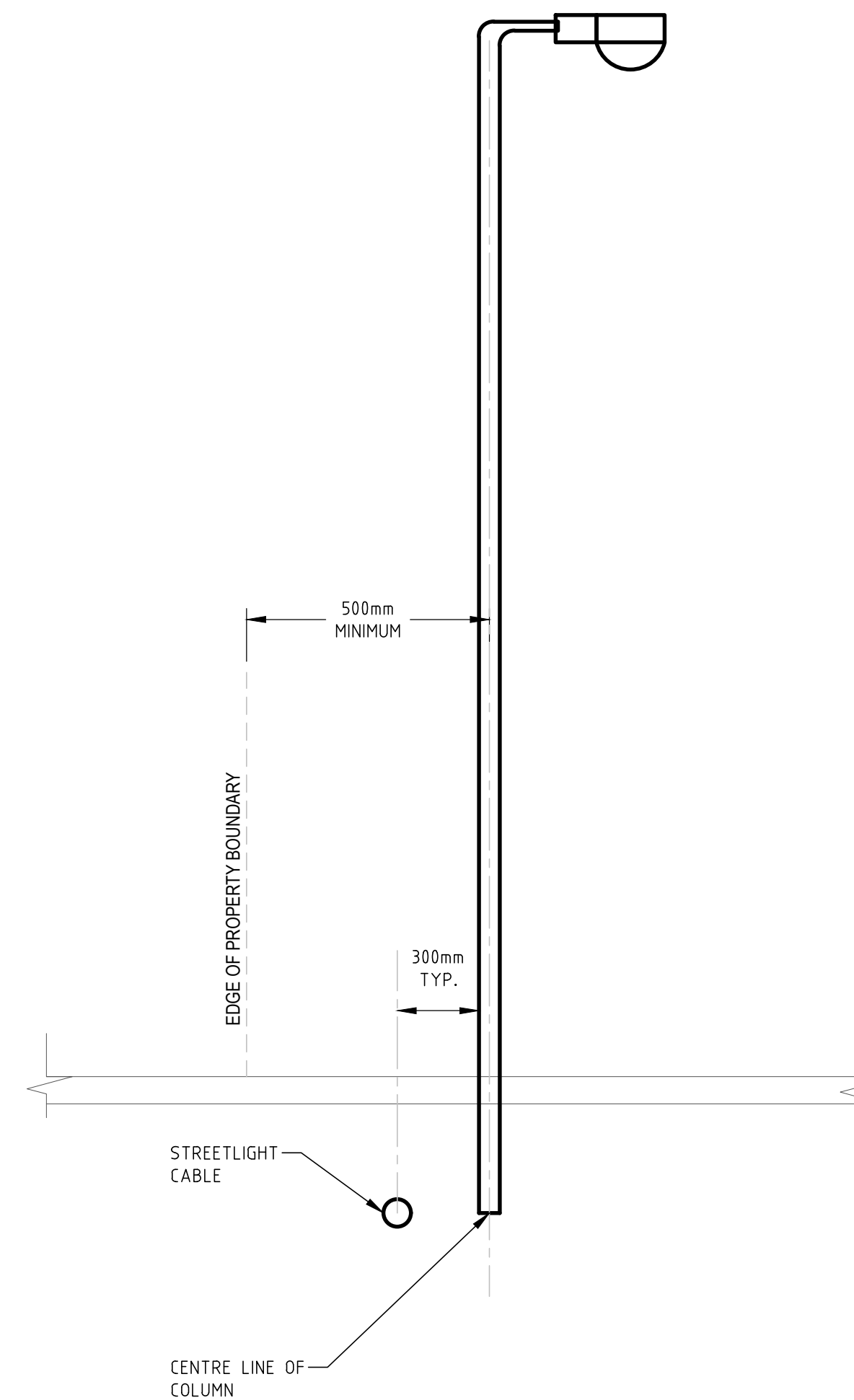
ADJACENT PROPERTY BOUNDARY
