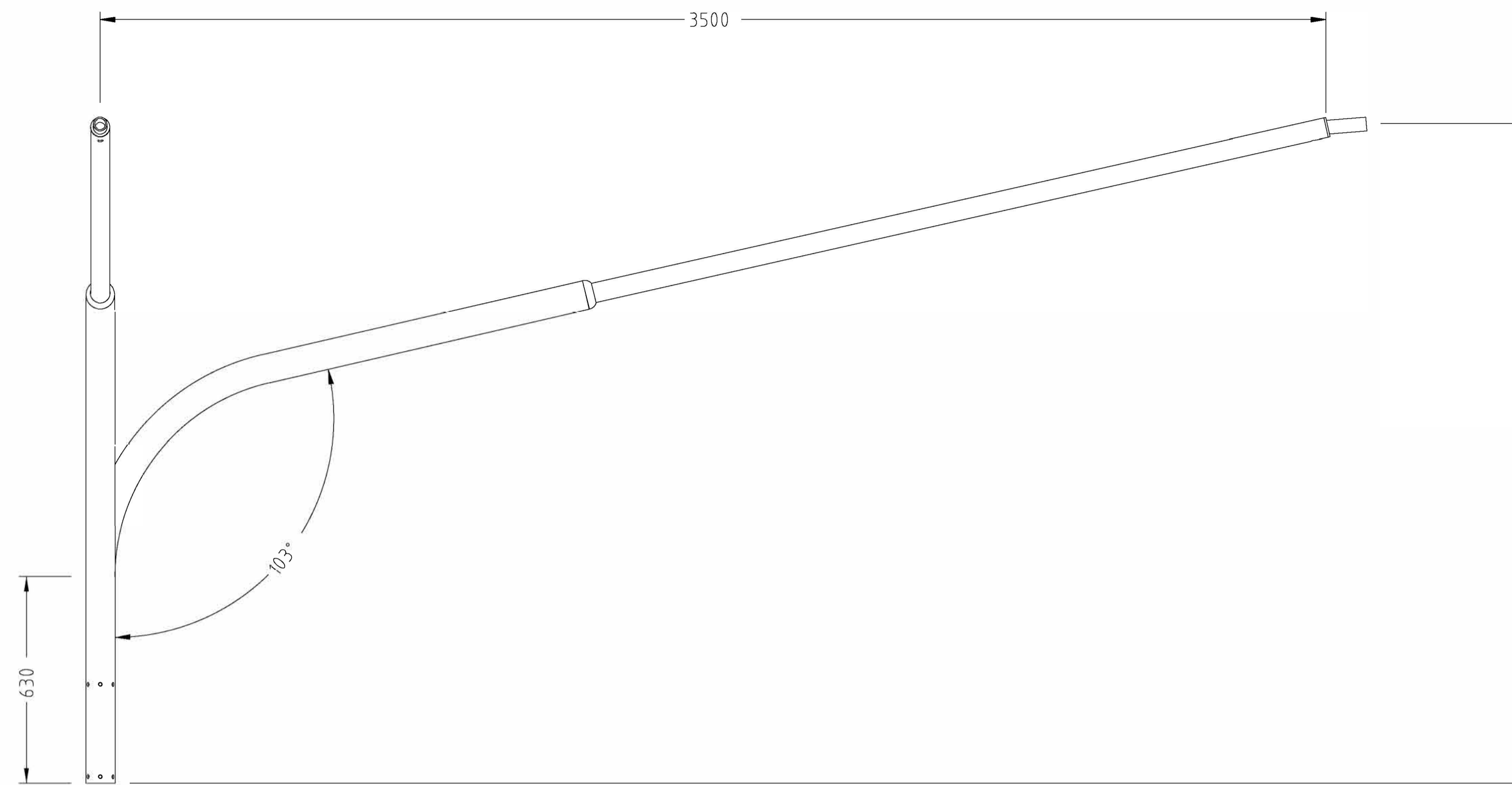
SIDE ELEVATION
